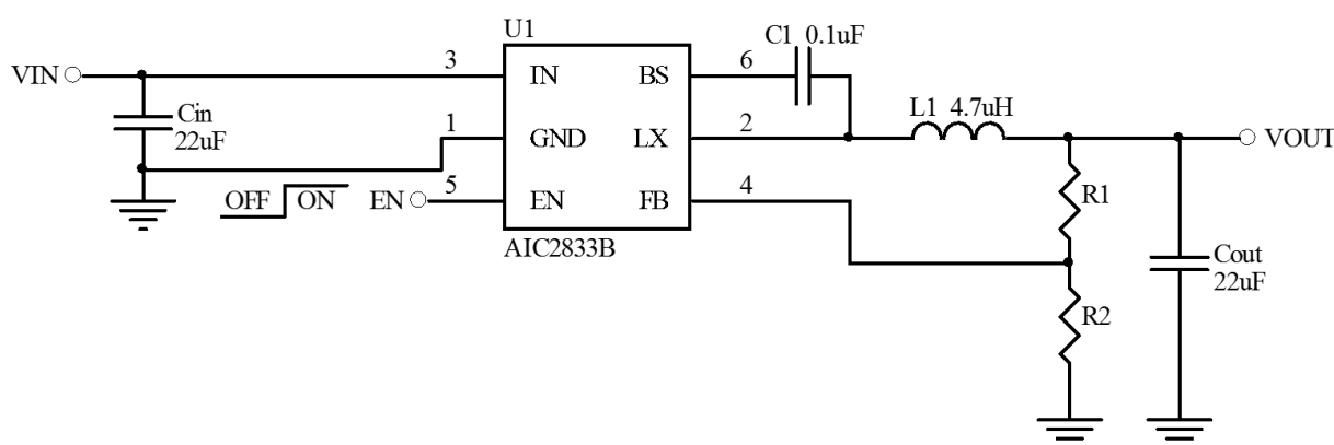
AIC2833B Typical Application Circuit
