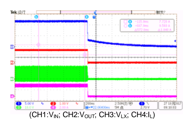
Fig. 6 Power Off at V_{IN}=12V , V_{OUT}=1.2V , I_{OUT}=2A
