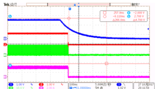
Fig. 10 Enable Off at V_{IN}=12V , V_{OUT}=1.2V , I_{OUT}=2A
