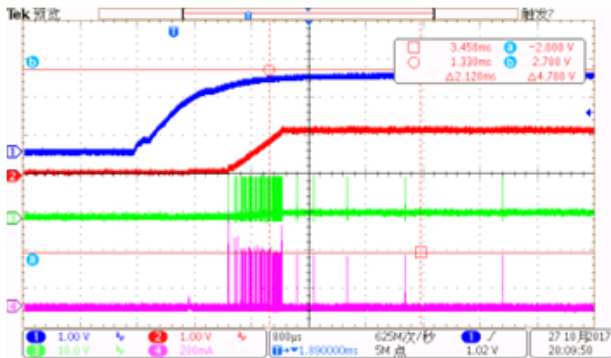
Fig. 7 Enable On at V_{IN}=12V , V_{OUT}=1.2V , I_{OUT}=0A
