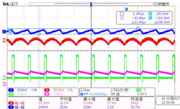
Fig. 13 Input/Output Ripple at V_{IN}=12V , V_{OUT}=1.2V , I_{OUT}=2A
