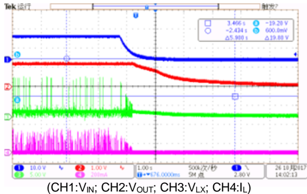
Fig. 4 Power Off at V_{IN}=12V , V_{OUT}=1.2V , I_{OUT}=0A
