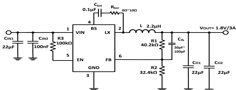
Figure 6. 12V IN , 1.8V/3A Output
