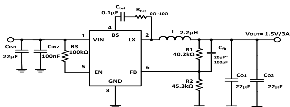
Figure 7. 12V IN , 1.5V/3A Output
