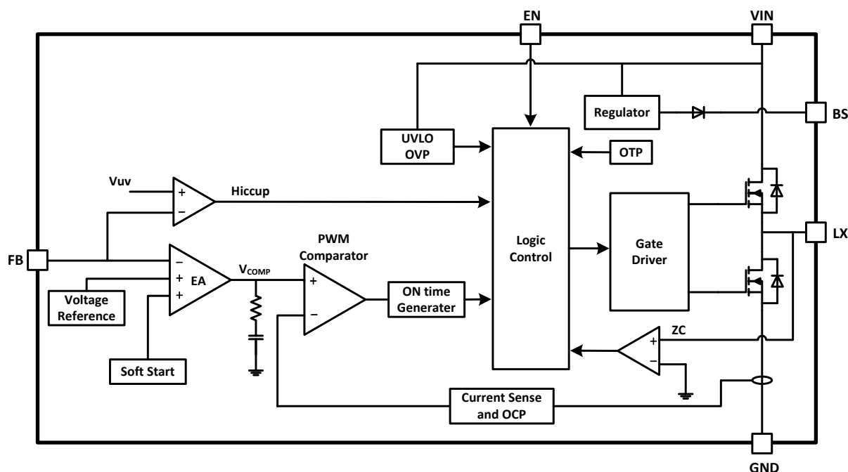
Figure 1. AIC2848B Block Diagram
