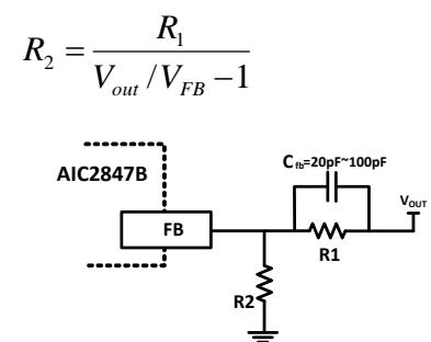
Figure 2. Feedback Network
