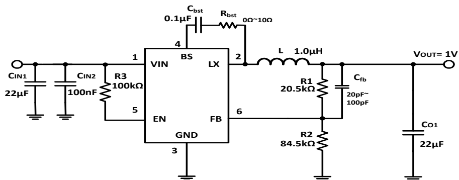
Figure 9. 12V IN , 1V/2A Output
