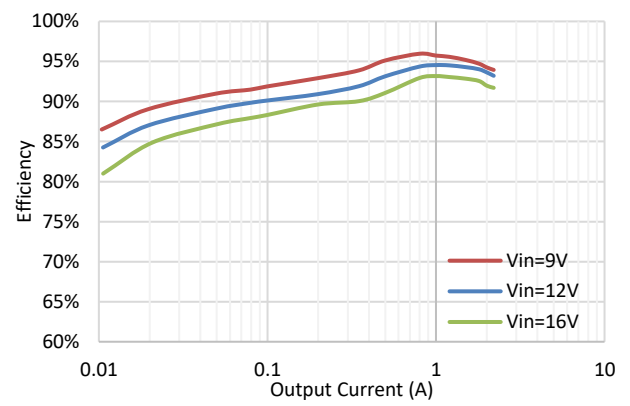
Efficiency at V_{OUT} = 5V
