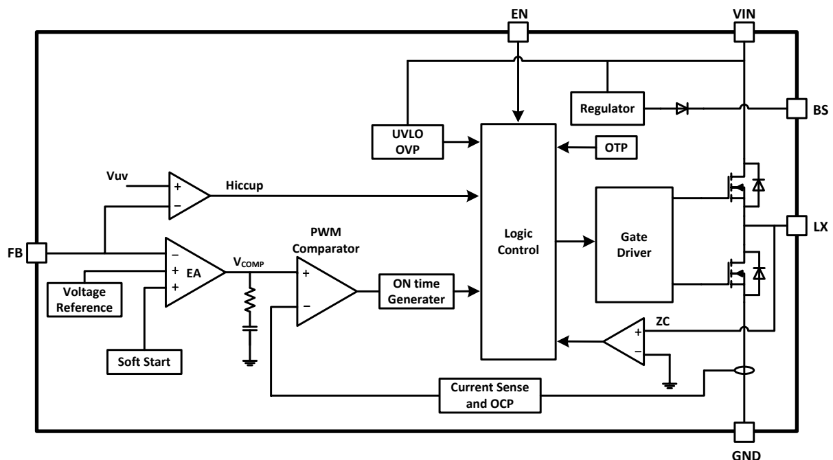
Figure 1. AIC2847B Block Diagram
